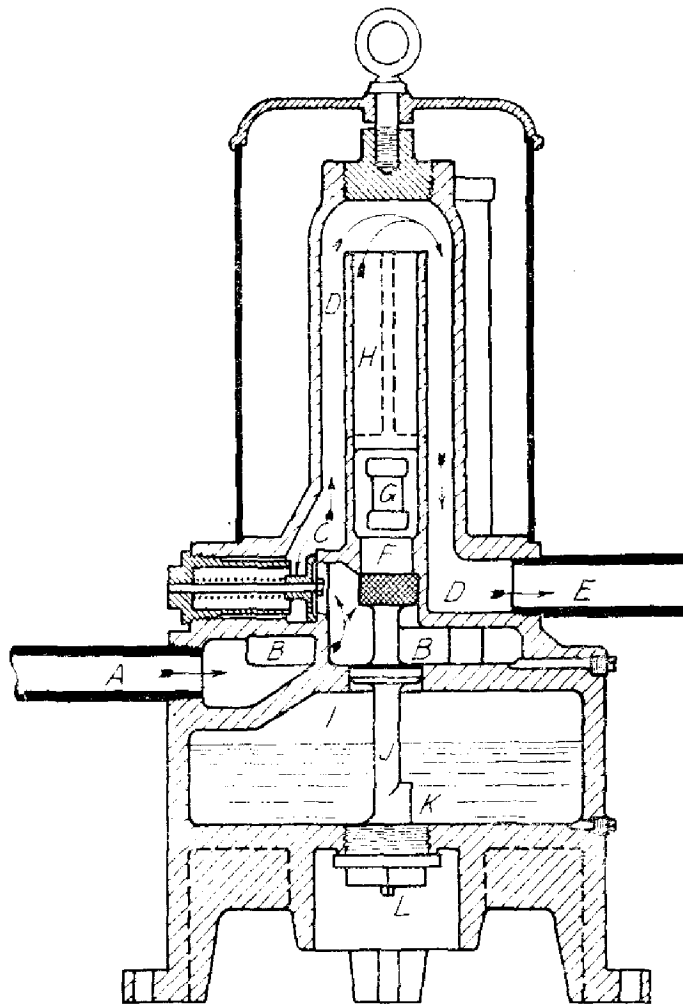
FIG. 6. SECTIONAL VIEW OF INTERNAL COMBUSTION REHEATER
